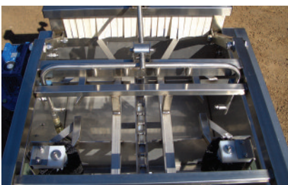
Top: Top and side brushes. Right: Fixed position jet system. Above: Williames Stainless Steel Tray Washer.
